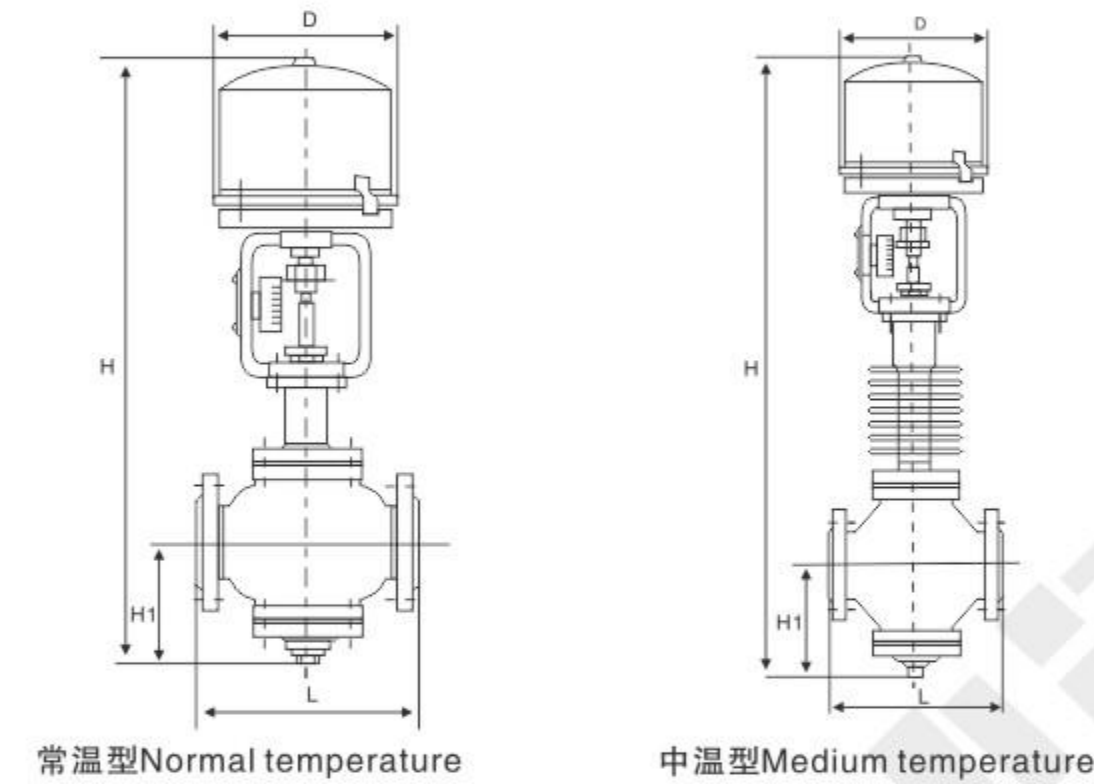
ZDLQ三通合流调节阀外形尺寸Three confluence regulating valve external dimensions
