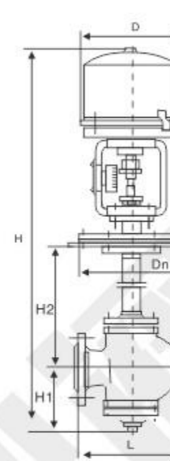
低温型Low temperature
