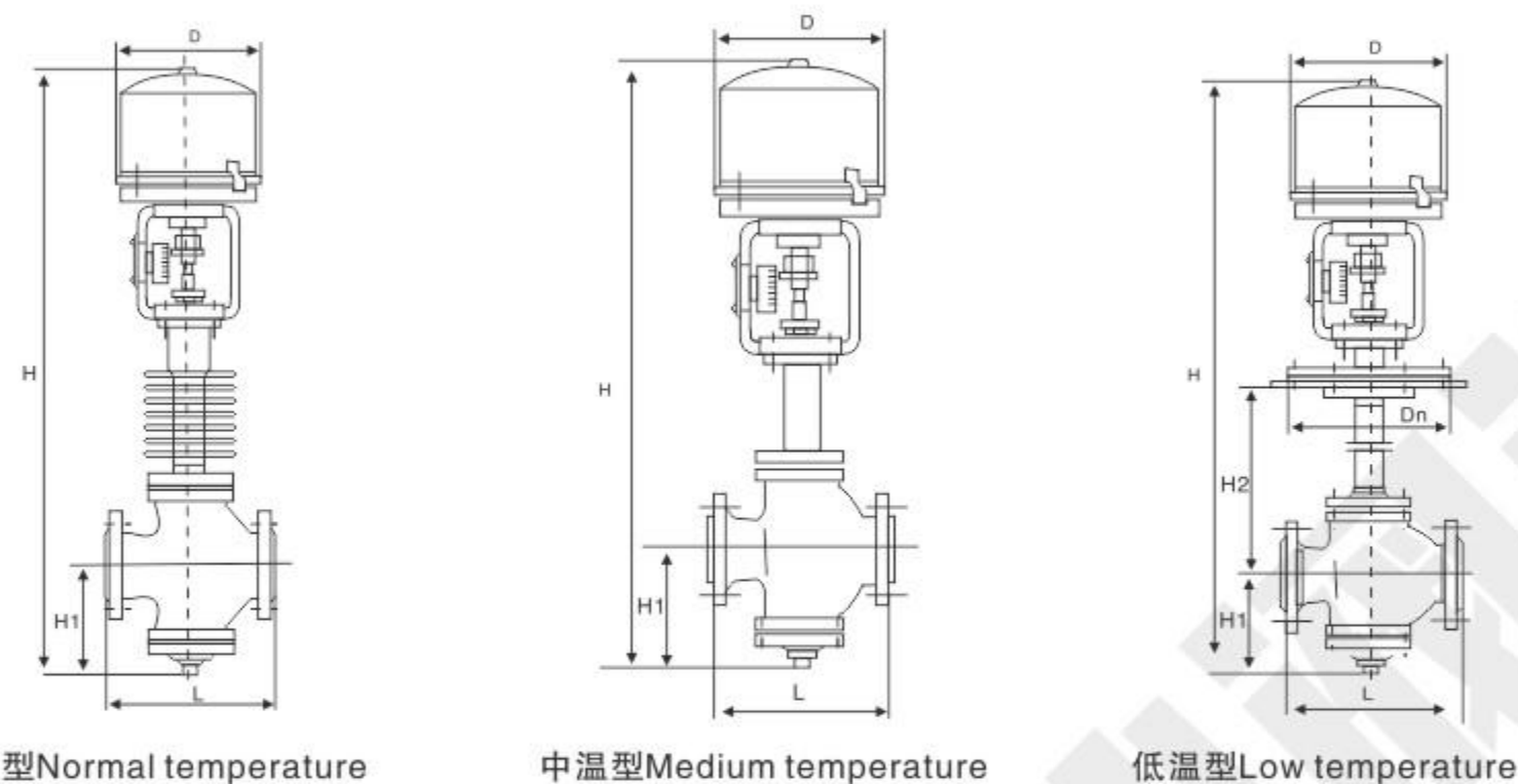
常、中温双座阀外形尺寸Normal, medium temperature double-seat valve external dimensions
