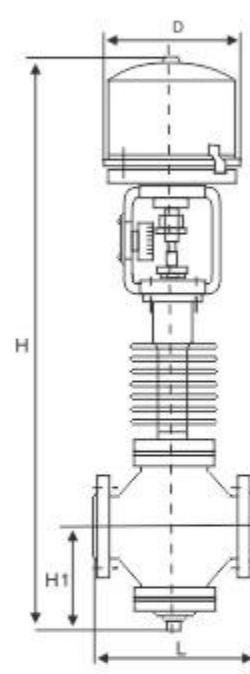
中温型Medium temperature
