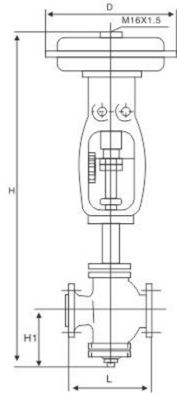
常温型Normal temperature
