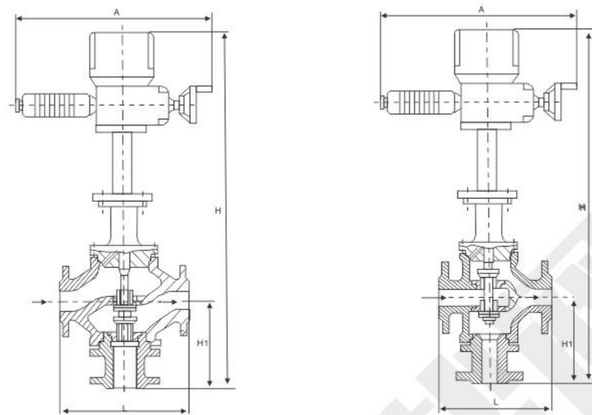
三通合流调节阀Three confluence regulating valve 三通分流调节阀Three shunt valve
